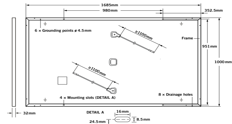
Fig. 1: External dimensions (in mm) and components for Q.PEAK DUO-G5.X, Q.PEAK DUO BLK-G5.X,
